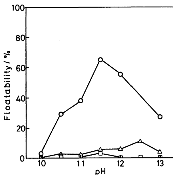
Fig. 8. Selective flotation of Cs + from a mixture of alkali metal ions. \circ : Cs + , \Delta : Rb + , \square : K + . Mixture: [Cs + ]=[Rb + ]=[K + ]= 7.5 \times 10^{-5} mol dm -3 , [Na + ]=0.1 mol dm -3 , 200 cm 3 . [4]Ar-R 12 : 3 \times 10^{-4} mol dm -3 .
